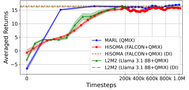
(b) Averaged Returns
