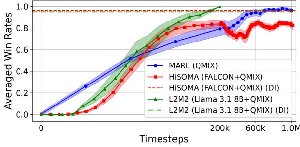
(a) Averaged Win Rates
